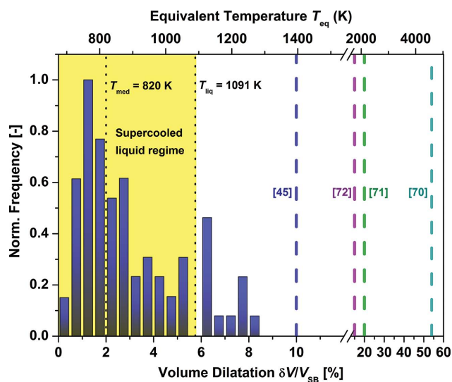
Figure 7. Histogram of volume dilatations \delta V/V_{SB} obtained from AE-pulses within the serrated flow regime for Vit105. [65] The majority of the \delta V/V_{SB} values falls within the domain of the equivalent supercooled liquid regime. All vertical dashed lines indicate values from previous ex situ works, [45,70–72] and the vertical dotted lines ( T_{med} = 820 \text{ K} and T_{liq} = 1091 \text{ K} ) show the equivalent temperature for the median volume dilatation and the equivalent liquidus temperature.
