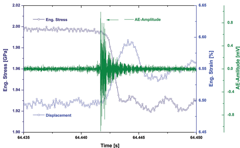
Figure 6. Stress drop and acoustic emission amplitude as a function of time for a Vit105 metallic glass tested at -10^{\circ}\text{C} at a strain rate of \dot{\epsilon} = 10^{-3} \text{ s}^{-1} (serrated flow regime). The emitted pulse appears at the onset of the stress drop. The corresponding jump in strain is also shown.
